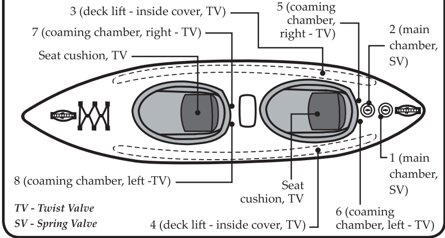
Diagram of Inflation Chambers
